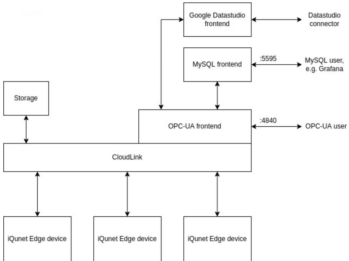
Figure 12: iQunet-CloudLink architecture
